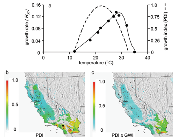
Fig. 7. The pathogen X. fastidiosa : (a) in vitro growth rate d^{-1} (R_{Xf}) (—) and normalized growth rate index ( PDI , - - -) on temperature (Feil and Purcell 2001), and the distribution of (b) mean PDI , and (c) mean PDI × GWI across California (see text for definitions of PDI and GWI ).
